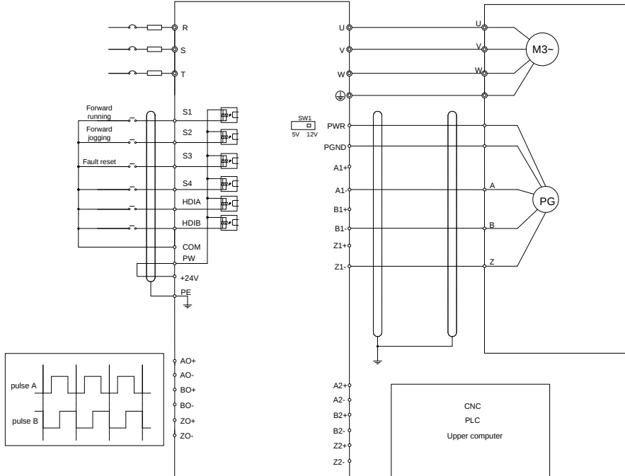
The following figure shows the external wiring of the expansion card used in combination with a differential encoder.
