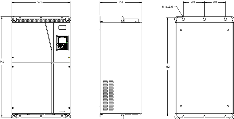
Figure C.7 132G/160P-200G/220P wall-mounting diagram
