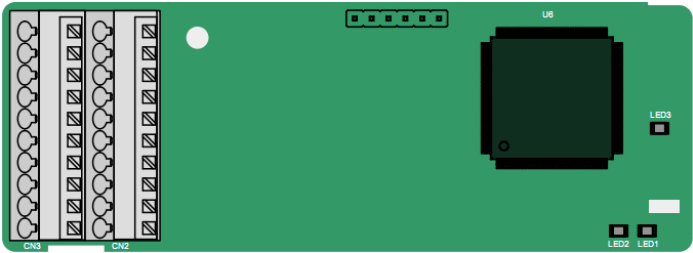
A.7.5 24V multi-function incremental PG card——EC-PG505-24
