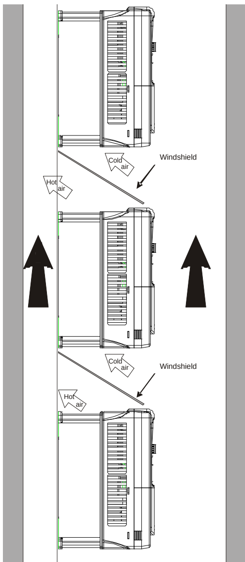
Figure 4.5 Vertical installation
