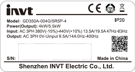
Figure 3.5 Product nameplate
