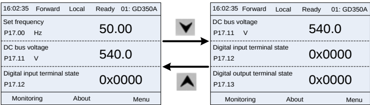
Figure 5.3 Stopped state parameters
