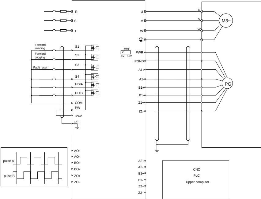
A.7.5 24V multi-function incremental PG card——EC-PG505-24
