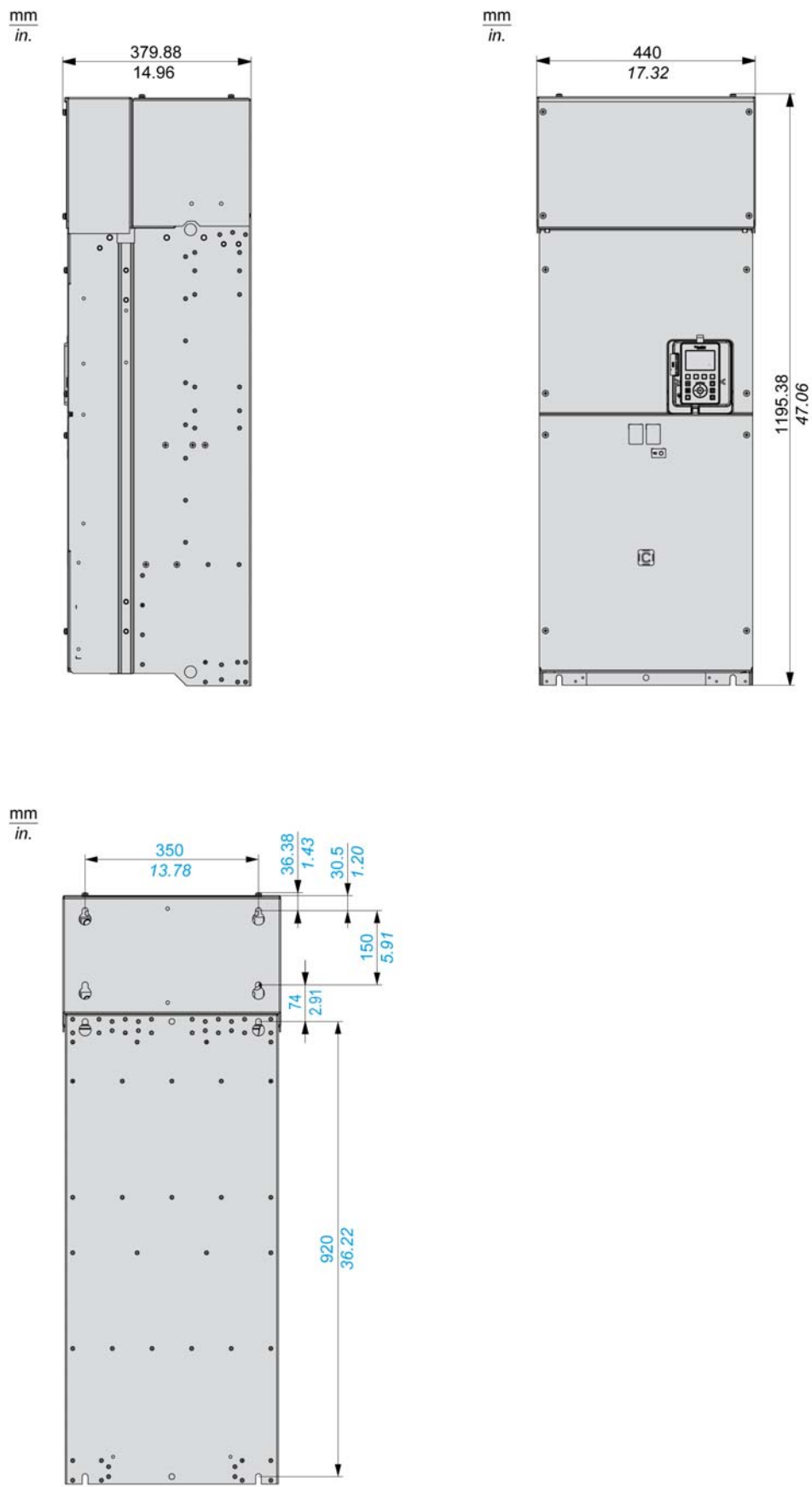
IP20 On Top and IP00 on bottom Drives - Side, Front and rear View
