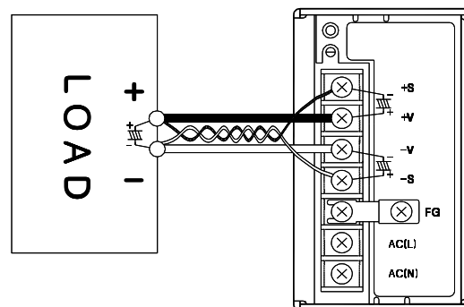
Fig 2. Remote sensing connection
