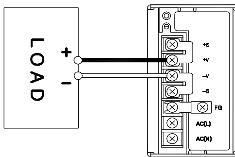
Fig 1. Basic connection
