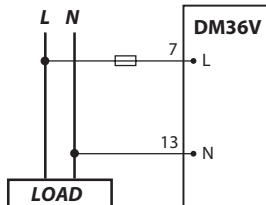
DM36V single-phase voltage measurement connection diagram.
