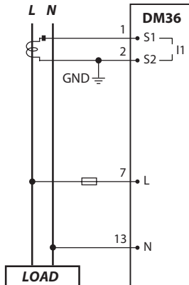
DM36 single-phase measurement connection diagram.
