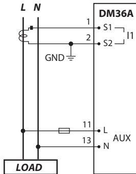
DM36A single-phase current measurement connection diagram.
