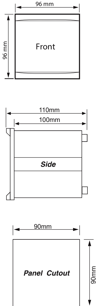
Figure 2: Case Dimension
