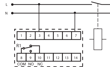
Single-Phase System
