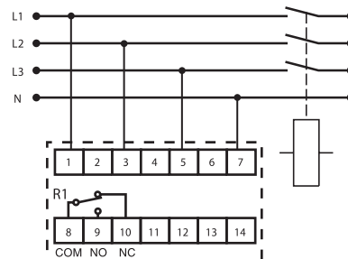
3-Phase System
