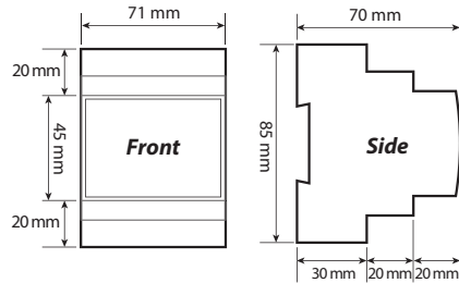
Figure 6: Case Dimensions
