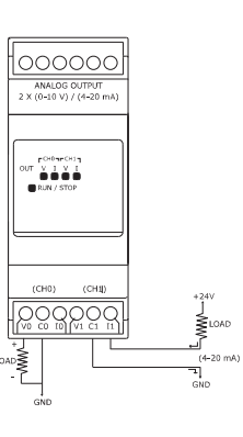
Connecting Analog Output Model
