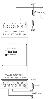
Connecting Analog Input Model
