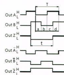
Line driver
