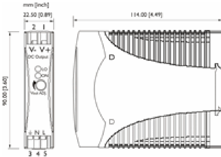
DIMENSIONAL DIAGRAM
