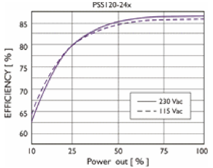
EFFICIENCY CURVE
