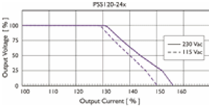
DERATING CURVE
