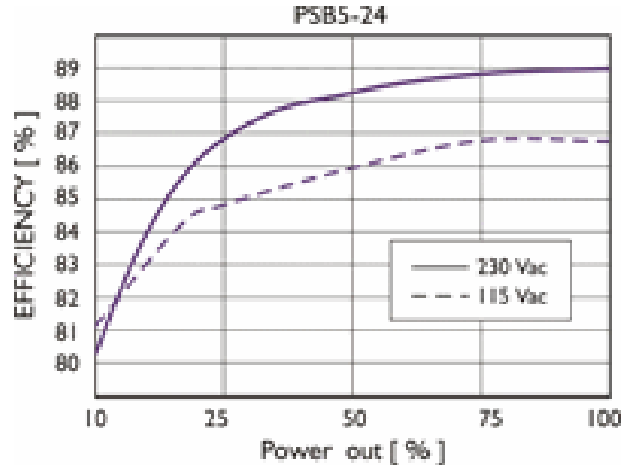
EFFICIENCY CURVE
