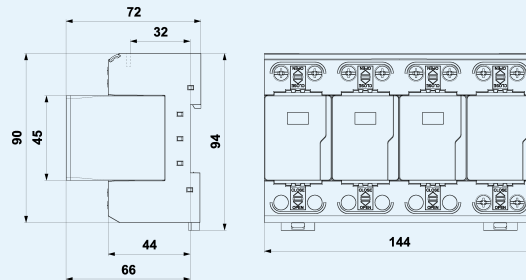
Product dimensions
