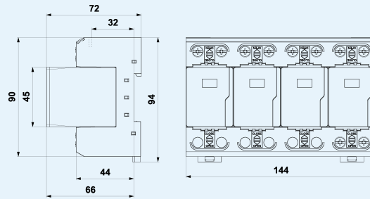
Product dimensions
