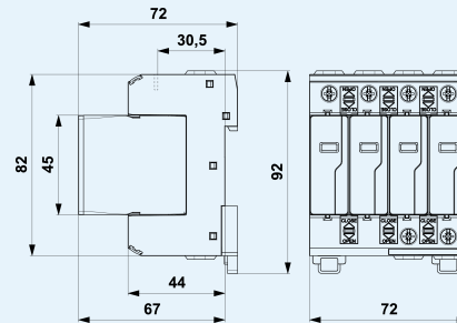
Product dimensions
