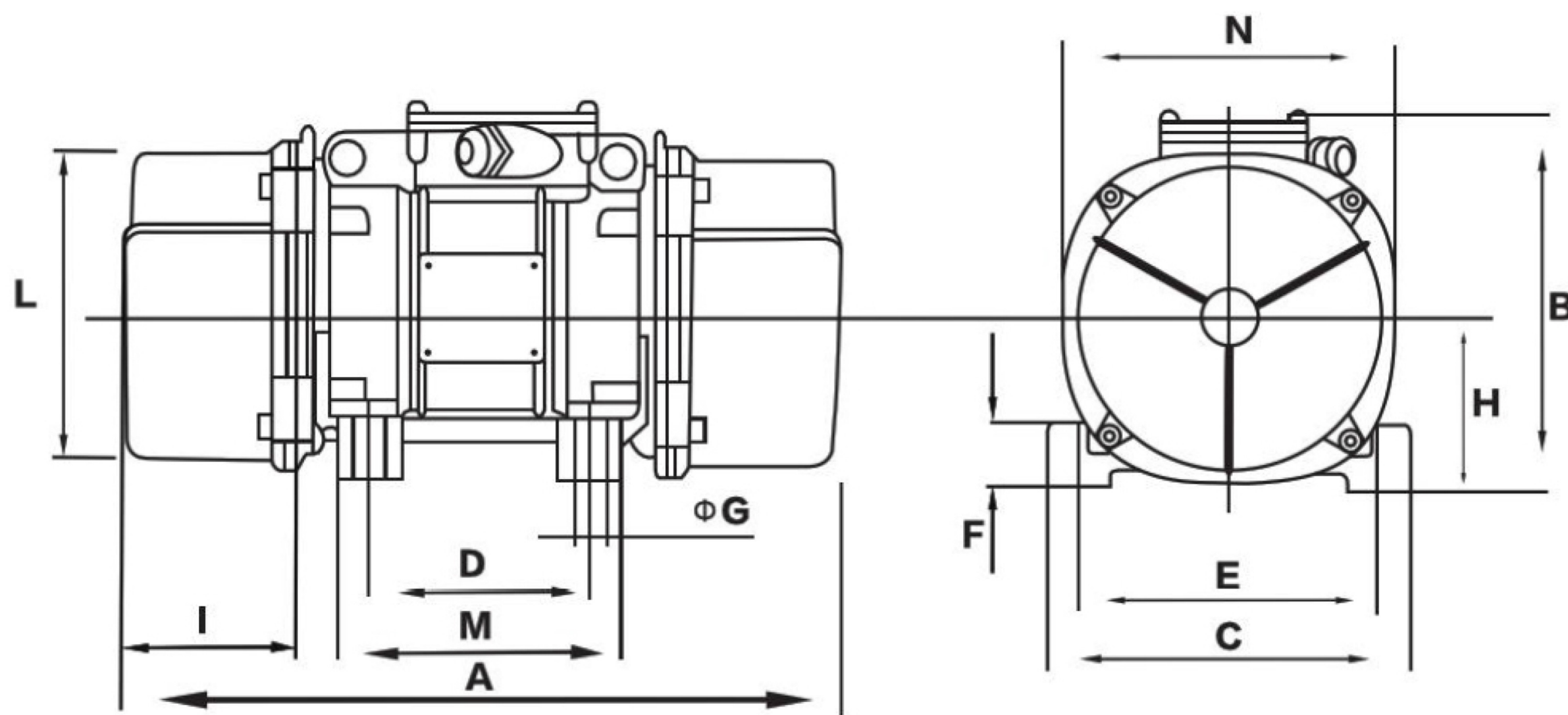
CVM SERIES DIMENSIONAL FEATURES
