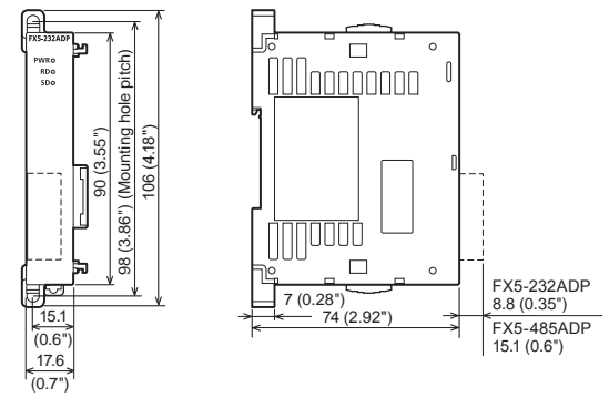
FX5-232ADP / FX5-485ADP
