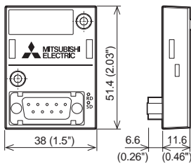
FX5-232-BD MASS (Weight): Approx. 0.02 kg (0.05 lbs)
