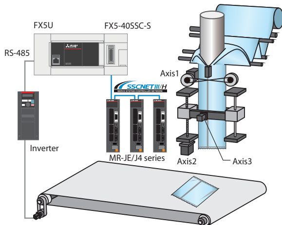
[Example of packaging machine using Simple Motion]
